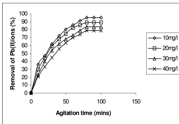
Figure 3. Effect of agitation time and initial Pb(II) ion concentration on adsorption of Pb(II) ions on to SCHC
