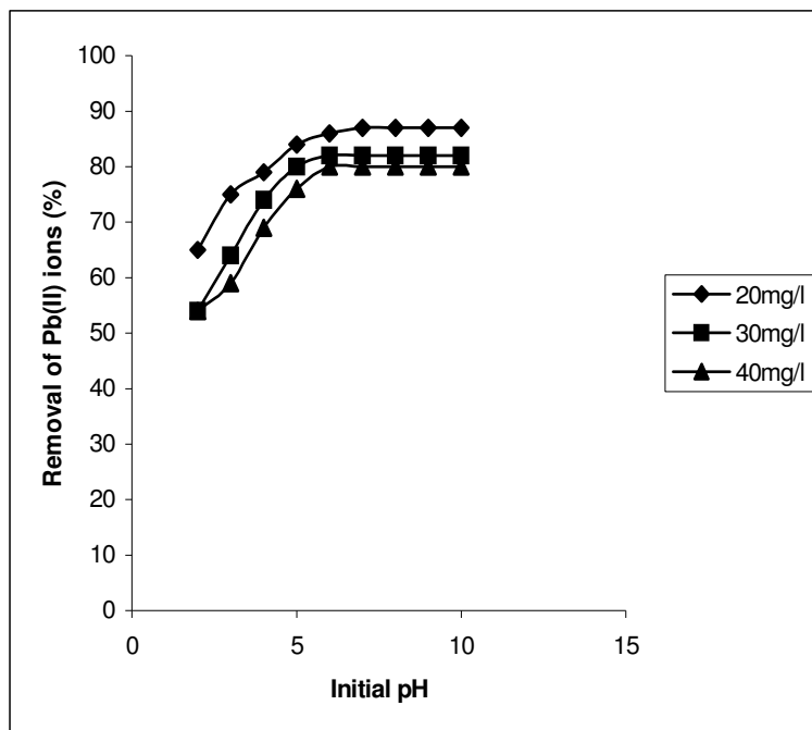
Figure 5. Effect of initial pH on the removal of Pb(II) ions from aqueous solution by SCH carbon
