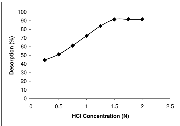
Figure 6. Desorption of Pb(II) ions from SCH carbon
