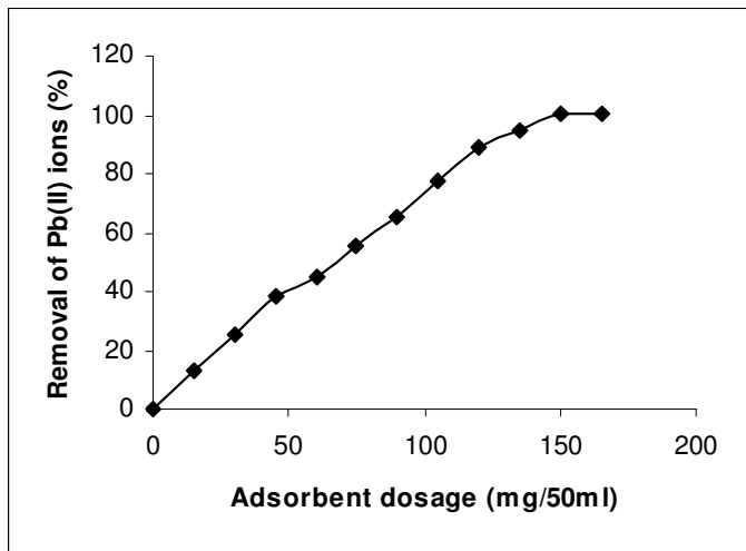
Figure 7. Effect of SCHC dosage on the adsorption of Pb(II) ions from radiator manufacturing industry waste water
