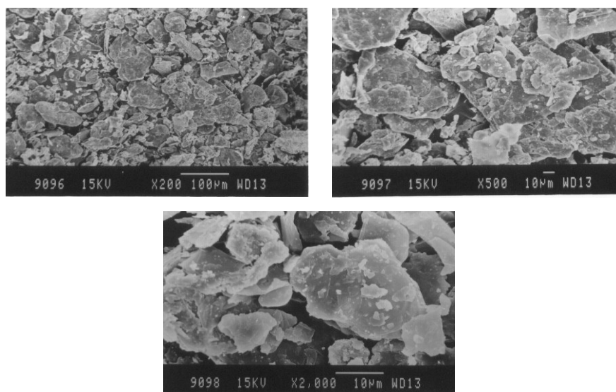
Figure 1. SEM photograph of Silk cotton hull activated carbon (SCH) at various magnifications (x200, x500 and x2000)
