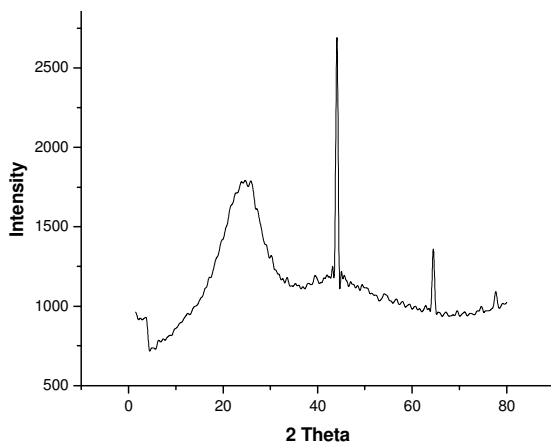
Figure 2. X-ray Diffraction pattern for SCH
