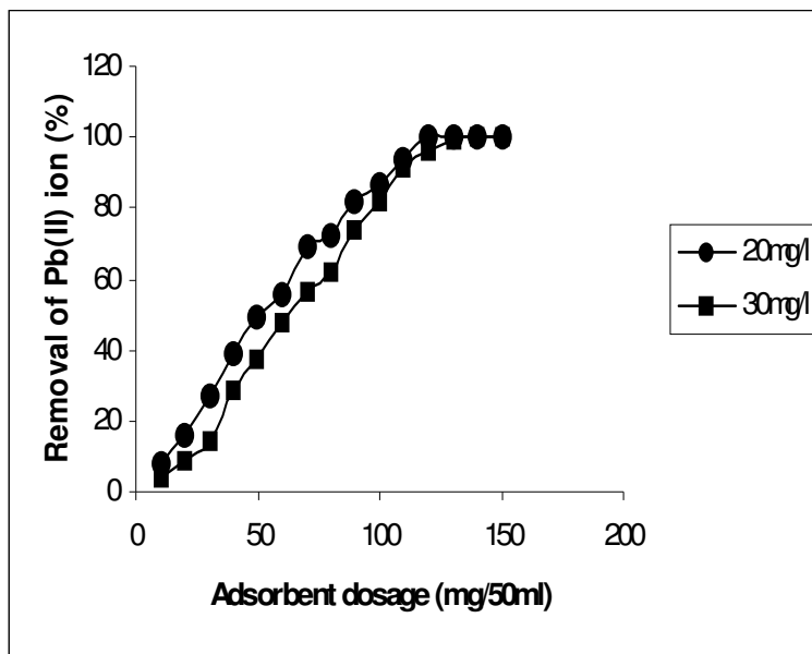
Figure 4. Effect of SCHC dosage on the adsorption of Pb(II) ions
